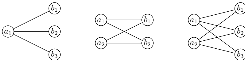
Obrázek A.2: Grafy S_3 = K_{1,3}, K_{2,2}, K_{2,3}
